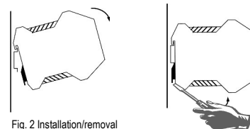
Fig. 2 Installation/removal
